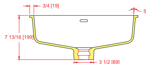
Section B-B
