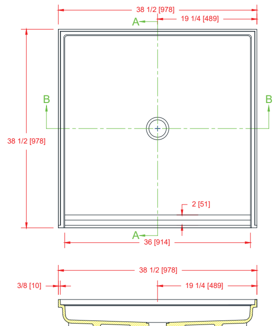
SECTION B-B
